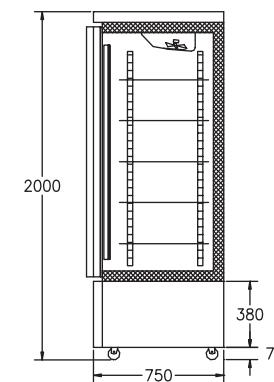
CROSS SECTION
